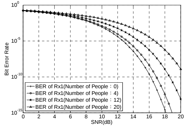
Figure 4. BER versus SNR for the different distribution of people
