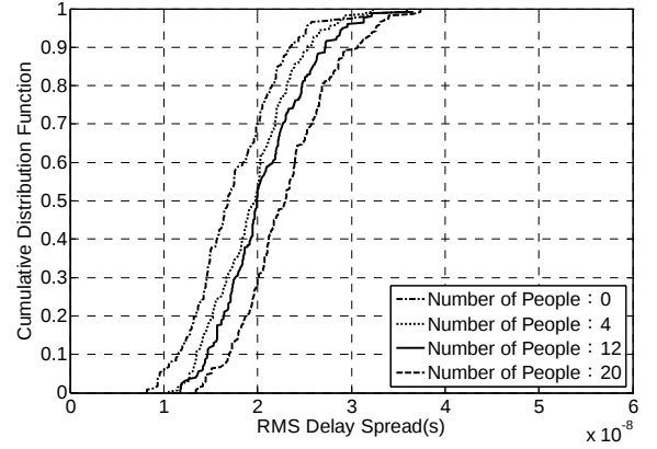
Figure 3. Cumulative distribution of RMS delay spreads for the different distribution of people
